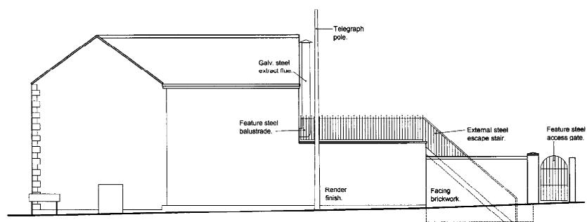
Side Elevation
