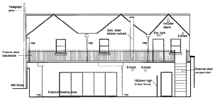
Rear Elevation
